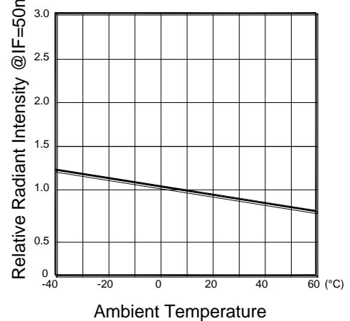
Fig.4 Relative Radiant Intensity Vs Ambient Temperature @ I_F=50\text{mA}
