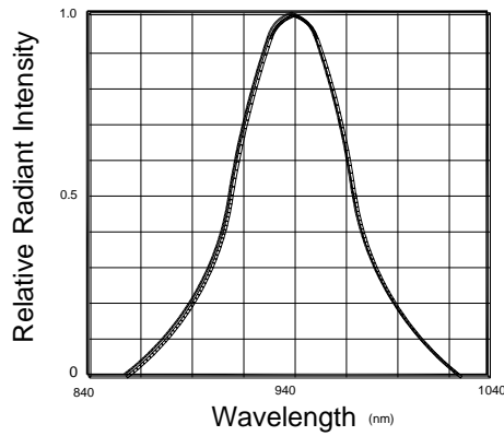
Fig.1 Spectral Distribution
