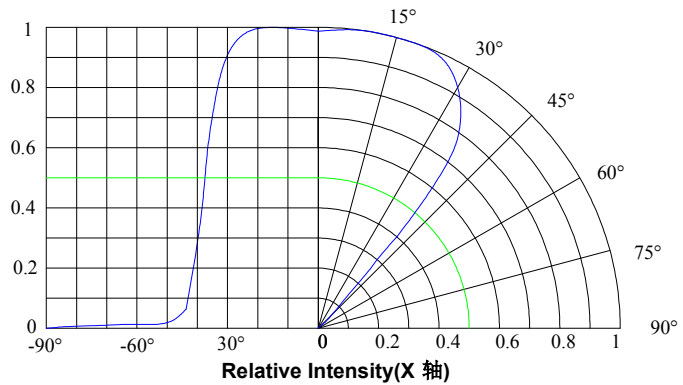
Fig.6 Radiation Diagram
